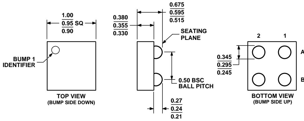
Figure 53. 4-Lead Wafer-Level Chip Scale Package [WLCSP] (CB-4) Dimensions shown in millimeters
