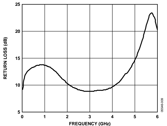
Figure 9. Return Loss vs. Frequency
